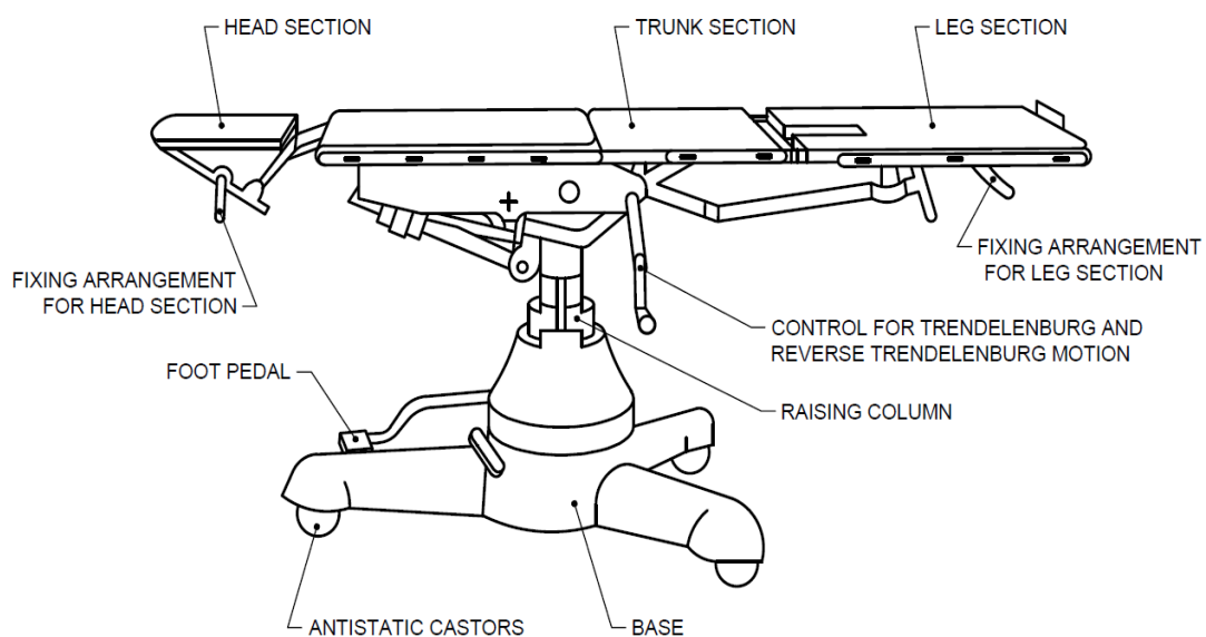
Fig. 1 PAEDIATRIC OPERATION TABLE
